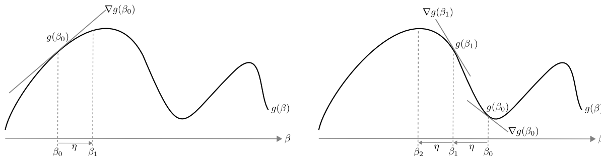
Figure 14.1: Start at some point \beta_0 . If the gradient is positive (left figure), try a larger value of \beta , say \beta_1 = \beta_0 + \eta . If the gradient is negative (right figure), try a smaller value of \beta , say \beta_1 = \beta_0 - \eta . Repeat this until convergence.
